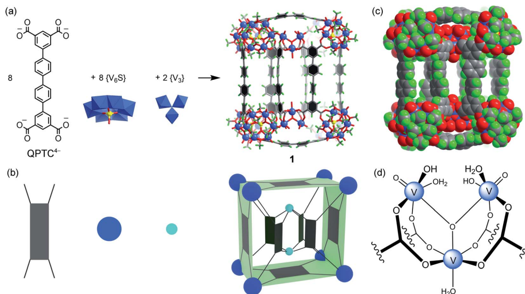
Fig. 1 (a) The self-assembly of 1 from \text{QPTC} linkers and \{\text{V}_6\text{S}\} and \{\text{V}_3\} SBUs; (b) a simplified cartoon model of 1 showing the ligand–node connectivities; the dark blue spheres represent the \{\text{V}_6\text{S}\} SBUs, the light blue spheres represent the \{\text{V}_3\} SBUs and the four-pronged rectangles represent the \text{QPTC} linkers; (c) the space-filling model of 1 illustrating the three compartments of its interior cavity (V blue; S yellow; O red; C dark gray; H green). Counter ions and solvent molecules are omitted for clarity; (d) chemical structure of the \{\text{V}_3\} SBU.
