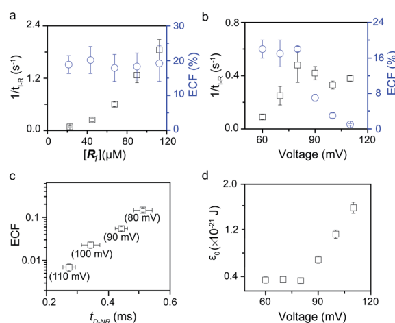
Fig. 2 Kinetics evaluation of \mathbf{R}_1 reacting with the K238C AeL nanopore. (a) The reaction rate ( f_{\text{PR}} = 1/t_{1-\text{R}} ) and fraction of effective collision (ECF) at different \mathbf{R}_1 concentrations. (b) Reaction rate ( f_{\text{PR}} ) and ECF under different voltages from +60 mV to +110 mV. (c) The relationship between the ECF and non-reaction event duration ( t_{\text{D-NR}} ). The voltage dependent results of t_{\text{D-NR}} and t_{1-\text{NR}} are shown in Fig. S5a and b,† respectively. (d) The collision threshold energy ( \epsilon_0 ) under different voltages from +60 mV to +110 mV. All data were acquired at 20.0 \pm 2.0 °C in 1.0 M KCl, 10.0 mM Tris, and 1.0 mM EDTA solution buffered at pH 8.0 in the presence of 50.0 μM \mathbf{R}_1 .
