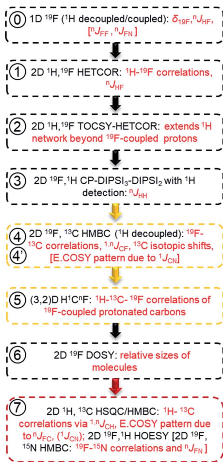
Fig. 5 Flow chart for acquiring and working with spectra of mixtures of fluorinated compounds. The information obtained is given in red. Golden and red boxes denote experiments involving ^{13}\text{C} , and the experiments for extending the structure beyond the F-containing moieties, respectively.
