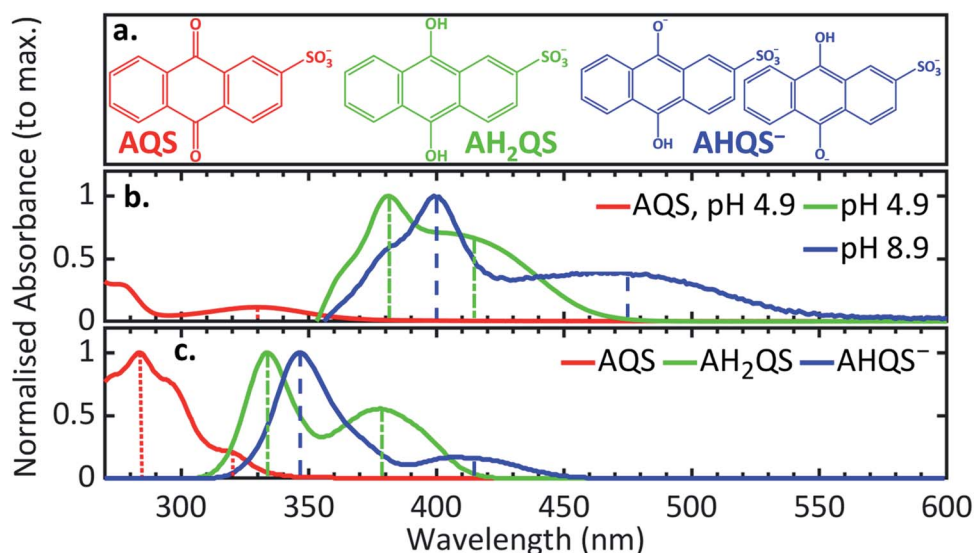
Fig. 7 (a) The structures of AQS and the species present at pH 4.9 and pH 8.9; (b) experimental UV/Vis spectra of AQS (0.1 M acetate buffer pH 4.9, 0.1 M PBS buffer pH 7.4, 0.1 M carbonate–bicarbonate buffer pH 8.9; 0.2 M KCl added in all solutions; ca. –0.65 V vs. SCE for 30 minutes before recording spectra); (c) the predicted UV/Vis spectra from the LC- \omega PBE explicit solvent TDDFT theoretical spectroscopy with spectral warp corrections applied (see ESI†). The vertical lines in (b, c) denote the experimental and theoretical peak positions corresponding to each feature. Note: the two structures studied for the species present at pH 8.9 showed very similar UV/Vis spectra.
