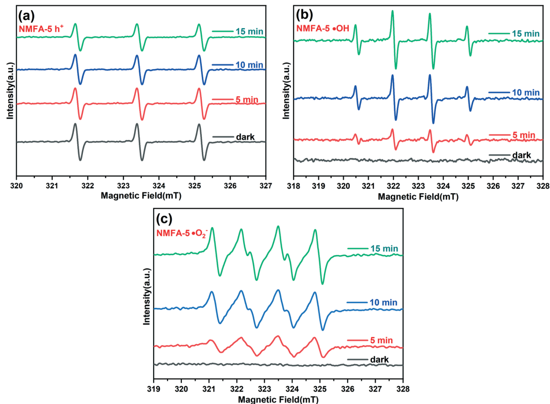
Fig. 14 The ESR spectra of (a) \text{h}^+ , (b) \cdot\text{OH} and (c) \cdot\text{O}_2^- generated using the NMFA-5 composites.
