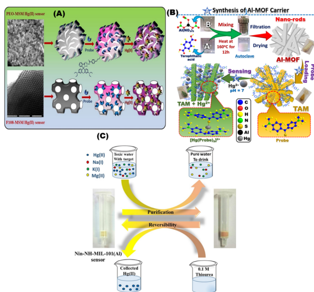
Fig. 7 (A) Schematic diagram for sensing Hg 2+ ions using bis(diethylamino)-3-oxospiro[isindoline-1,9'-xanthen]-2-ylcarbamothioyl)-4-butylbenzamide (BOICB) probe. 94 (B) Schematic representation of fabrication of nanorod TAM optical chemosensors and interactions with Hg 2+ ions under optimum conditions. 95 (C) Representative design of the Nin-NH-MIL-101(Al) sensor applied for purification of water polluted with Hg(II) ions and the reversible process by using 0.1 M thiourea solution (which can be repeated several times). 96 Reproduced with permission from ref. 94–96.
