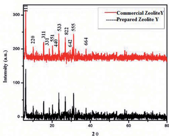
Fig. 3 X-ray diffraction patterns of commercial and prepared zeolite-Y.
