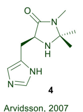
Scheme 4 Conjugate additions using pyrrolidines and imidazolidine catalysts.
