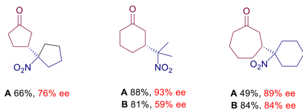
Scheme 3 L-Proline and its rubidium salt in the reaction with cycloalkenones.
