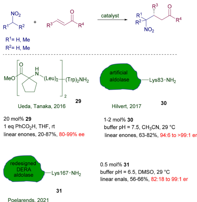
Scheme 22 Chiral peptide foldamers and aldolases as biocatalysts.
