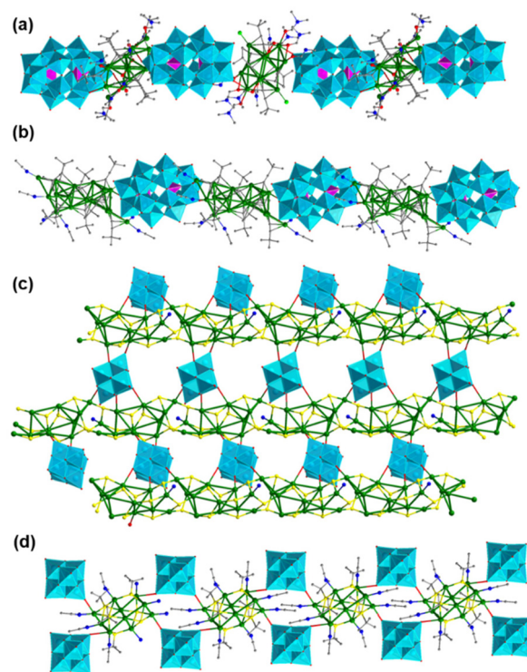
Fig. 16 Packing diagram of (a) \{[\text{Ag}_{14}(\text{C}\equiv\text{C}'\text{Bu})_8(\text{C}_3\text{H}_7\text{NO})_{10}][\text{Ag}_{12}(\text{C}\equiv\text{C}'\text{Bu})_6\text{Cl}(\text{DMF})_{10}]\text{H}[\text{P}_2\text{W}_{18}\text{O}_{62}]_2\}_n , (b) \{[\text{Ag}_{16}(\text{C}\equiv\text{C}'\text{Bu})_{11}(\text{CH}_3\text{CN})_6][\text{P}_2\text{W}_{18}\text{O}_{62}]\}_n , (c) \{[\text{Ag}_{11}(\text{tBuS})_9(\text{CH}_3\text{CN})][\text{Mo}_6\text{O}_{19}]\}_n and (d) [\text{Ag}_{10}(\text{S}'\text{Bu})_6(\text{CH}_3\text{CN})_8(\text{Mo}_6\text{O}_{19})_2]_n .
