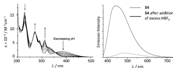
Fig. 12 (Left): evolution of UV–vis absorption spectrum of 55 upon addition of \text{HBF}_4 in 0.1 M aqueous NaCl solution at 298 K; (right): emission spectrum of 54 in \text{MeCN} at 298 K ( \lambda_{\text{ext}} 350 nm) before and after addition of excess \text{HBF}_4 . Adapted with permission from ref. 108. Copyright (2001) Elsevier Ltd.
