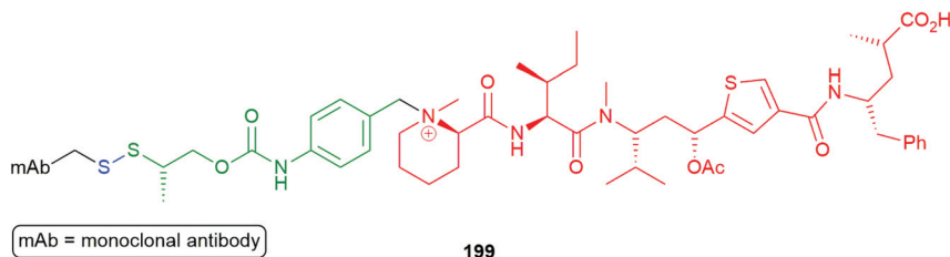
Fig. 12 Pillow's glutathione triggered antibody-double linker-drug conjugate 199 . 94
