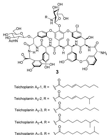
Fig. 8 Formula of teichoplanin 3 which is composed of a mixture of structural analogues. Each carries a different lipophilic moiety attached to the glucosamine residue.
