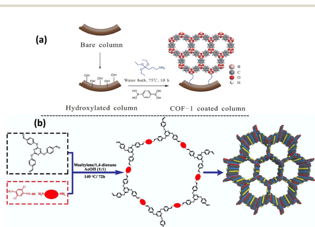
Fig. 3 A schematic diagram for the development of (a) Boron-based COF and (b) Triazine-based COF. Adapted with permission from ref. 54. Copyright © 2021 Elsevier B.V. All rights reserved; ref. 62. © 2021 Elsevier Ltd. All rights reserved.
