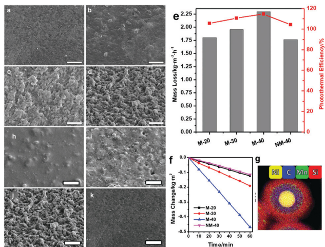
Fig. 6 SEM images of the \text{Ni}_{40}\text{C}_{20}/\text{PVA} composite film, with (a) 0 mT, (b) 100 mT, (c) 200 mT and (d) 400 mT magnetic field applied during the gelation process and the SEM images of (h) M-20, (i) M-30, (j) M-40 and (k) NM-40 (scale bar = 50 \mu\text{m} ). (e) The evaporation rates and energy conversion efficiencies of different films. (f) Water mass changes over time without light illumination at 20 ^{\circ}\text{C} on various films. (g) EDX mapping image of \text{Ni}@\text{RF}@\text{SiO}_2 core-shell nanoparticles. Reproduced with permission. 159 Copyright 2021, John Wiley and Sons.
