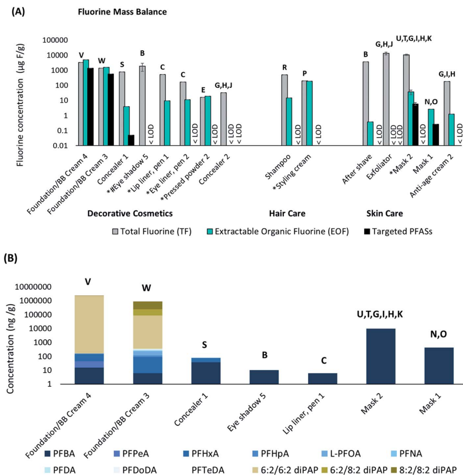
Fig. 3 (a) Fluorine mass balance showing TF, EOF and targeted PFAS concentrations ( \mu\text{g F g}^{-1} sample). The targeted PFAS ( \sum PFAS) concentrations were converted to fluorine concentrations for comparative purposes. ( \text{LOD}_{\text{TF}} = 35.45 \mu\text{g F g}^{-1} , \text{LOD}_{\text{EOF}} = 0.32 \mu\text{g F g}^{-1} , \text{LOD}_{\sum\text{PFAS}} = 0.0015 \mu\text{g F g}^{-1} ). *Mica listed among ingredients; #synthetic fluorophlogopite listed among ingredients. (b) Concentrations ( \text{ng g}^{-1} sample) of targeted PFAS in 5 decorative cosmetics and 2 skin care samples (masks). Samples not shown (8 out of 15) were <\text{LOD} . Samples are plotted on a logarithmic scale (base 10) to enhance readability. The letters on top of each bar correspond to structures provided in Fig. 2.
