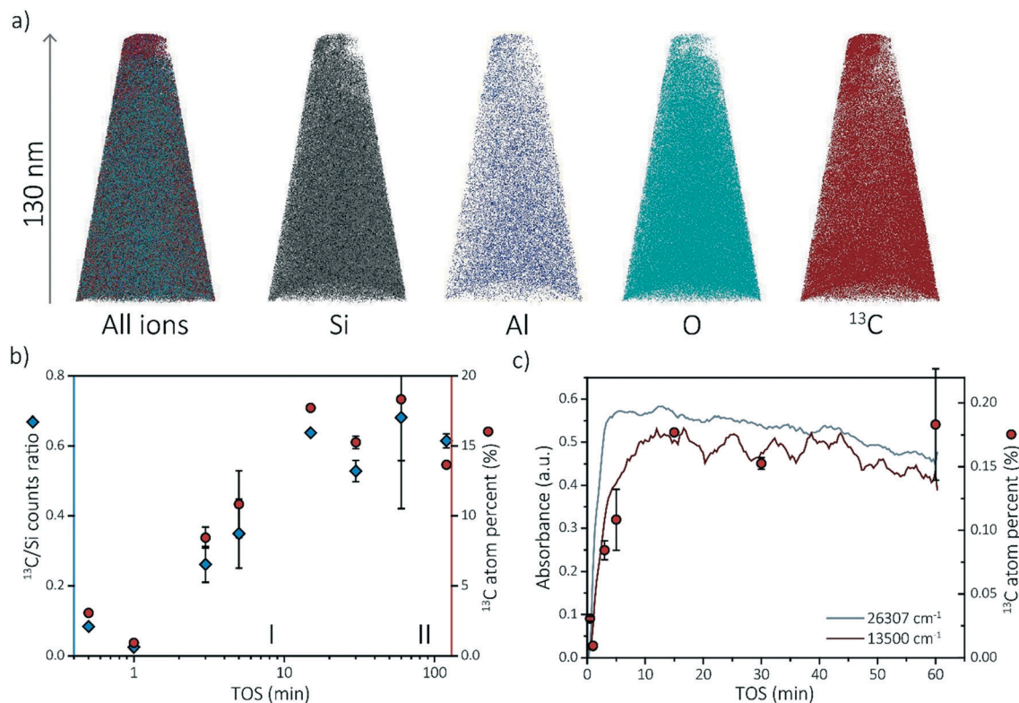
Fig. 3 a) Reconstructed needle (ion map of framework and coke molecule ions) of the 3 min coked H-SSZ-13 sample (2). b) The average ^{13}\text{C}/\text{Si} counts ratio and ^{13}\text{C} atomic fraction for the reconstructed needles as a function of time-on-stream (TOS) on a log-scale to amplify on the first reaction stage. c) The carbon content found with atom probe tomography compared to two different wavelength intensity evolutions of the single crystal UV-vis microscopy experiments showing similar trends. The 120 min has been left out for clarity reasons. For the 1 min and 15 min time-on-stream sample, only one needle has been reconstructed so no error bars are available.
