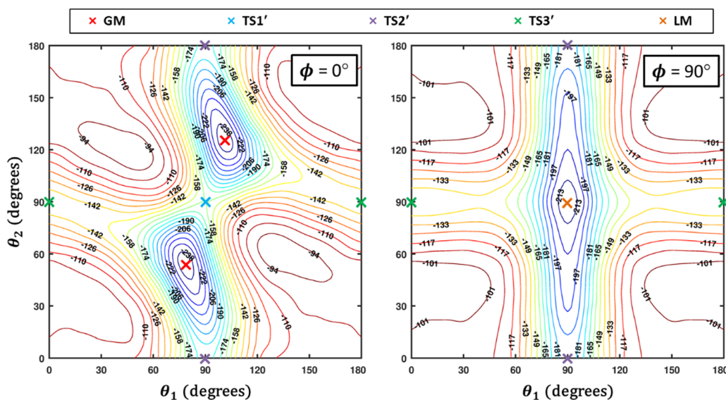
Fig. 3 R -Optimized contour plots of the CO 2 -O 2 4D-PES as a function of \theta_1 and \theta_2 for (at left) the planar ( \phi = 0^\circ ) geometries, and (at right) the non-planar ( \phi = 90^\circ ) geometries. For each pair of angles (\theta_1, \theta_2) , the energy is minimized by varying R . The global minimum (GM) and its symmetry partner appear in the \phi = 0^\circ plot at left, while the local cross-shaped minimum (LM) is found in the \phi = 90^\circ plot. Symmetry partners of the three second-order saddles (structures given in Fig. 1) are also indicated on the plots. The TS connecting GM and LM does not appear since \phi = 70.5^\circ for that structure (see Fig. 4).
