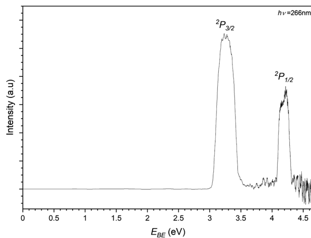
Fig. 8 Photoelectron spectrum of the 169 m/z peak from Fig. 3 assigned to photodetachment to the perturbed ^2P_{3/2} and ^2P_{1/2} states of the \text{I}^{\cdot-}\cdots\text{C}_3\text{H}_6 complex.
