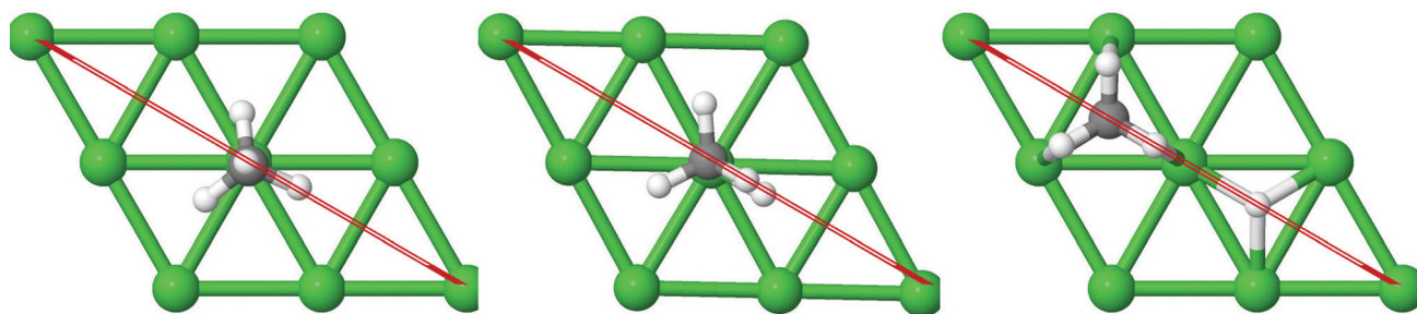
Fig. 4 The plane perpendicular to the Ni9/Pt(111) alloy, containing the carbon atom, dissociating hydrogen atom and one of the methyl hydrogen atoms. It can be seen from this figure that the reaction path for the dissociation of CH 4 is symmetric with respect to reflection through the plane shown in red. Here only the top layer of the alloy is shown. In Fig. 1(c) the optimized structures of Ni9/Pt(111) are shown with all the four layers as used in the calculation. Green balls in this figure refer to the nine Ni atoms present on the top layer of Ni9/Pt(111), and black and white balls refer to carbon and hydrogen atoms, respectively.
