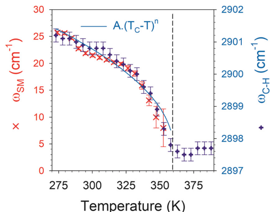
Fig. 6 Combination of low- and high-frequency Raman analyses. Comparison of the temperature dependence of the C–H stretching band frequency at 2900 cm −1 with that of the soft mode; symbols result from fitting procedures of lattice modes and C–H stretching spectra, and the line corresponds to the fitting procedure of C–H stretching frequencies with the function A \cdot (T_C - T)^n with T_C = 360 K. The fitting procedure is converging towards the parameters: A = 0.39 \pm 0.06 and n = 0.51 \pm 0.04 ( R = 0.977 ).
