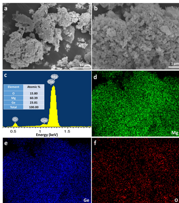
Fig. 4 SEM characterisation of \text{Mg}_2\text{Ge} powders synthesised from Mg and Ge at 200 W with an irradiation time of 60 s, showing: (a and b) SEM images at different magnification; (c) a representative EDX spectrum taken from the area shown in the image in (b); and (d–f) elemental maps of Mg, Ge and O, respectively, taken from the same area shown in (b).
