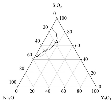
Fig. 1 Glass formation range in units of [mol%] in the system \text{Na}_2\text{O} – \text{Y}_2\text{O}_3 – \text{SiO}_2 reported in ref. 4 (solid line) and ref. 2 (dashed line). The dot depicts the starting composition for the investigations within this manuscript.
