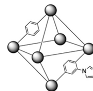
Fig. 1 Schematic structure of mixed-linker MOF 1 ; grey spheres represent [\text{Zr}_6(\mu_3\text{-O})_4(\mu_3\text{-OH})_4(\text{CO}_2)_{12}] units, connected by BDC or BDC-Im linkers.
