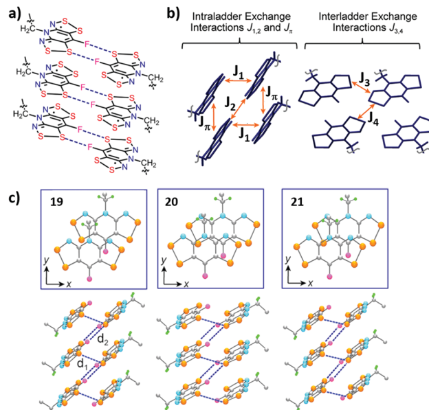
Fig. 18 (a) Bisdithiazolyl radical intermolecular \text{S} \cdots \text{F} contacts (supramolecular synthons) that lock radicals laterally into centrosymmetric pairs. (b) Pairwise exchange interactions J_1 , J_2 , J_3 , J_4 , and J_\pi . (c) In the top, slippage of adjacent radicals in 19–21 along the \pi -stacks in local coordinates x and y . In the bottom the ladder-like packing and contacts d_1 ( \text{S} \cdots \text{S} ) and d_2 ( \text{F} \cdots \text{S} ) connecting paired stacks. For clarity, the alkyl chains have been truncated after C2. Adapted with permission from ref. 72. Copyright 2013 American Chemical Society.
