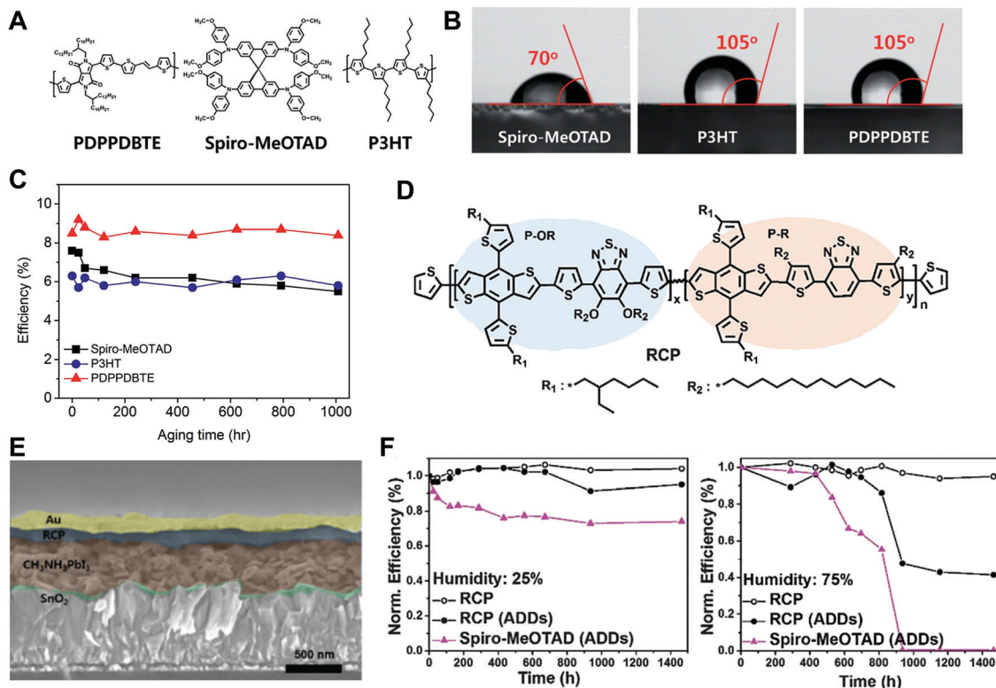
Fig. 4 Chemical structure of three common HTMs used in PSCs (A). Water contact angles associated with spiro-OMeTAD, P3HT, and PDPPDBTE HTLs (B). PCE stability associated with each HTL when used in unencapsulated PSCs at 20% RH (C). Reproduced with permission from ref. 30. Copyright 2014 The Royal Society of Chemistry. The chemical structure of the dopant-free RCP HTM. (D). A cross-sectional SEM image depicting the structure of the PSC. (E) Stability testing results of PSCs using the dopant-free RCP HTM, the doped RCP HTM, and doped spiro-OMeTAD at 25% RH. The initial efficiency was 17.3%. (F) The same stability results at 25% and 75% RH. Reproduced with permission from ref. 28. Copyright 2016 The Royal Society of Chemistry.
