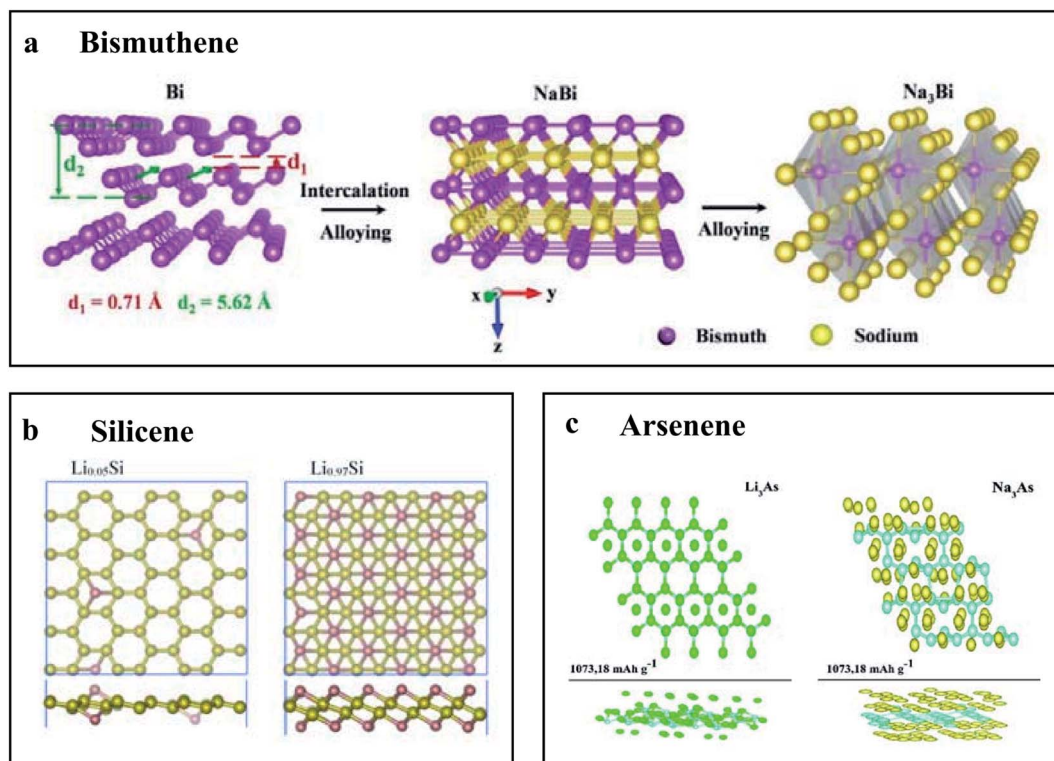
Fig. 4 Schematic diagram of structure evolution of elemental 2D materials during the operation of a Li-ion battery and Na-ion battery. (a) Schematics of structural evolution of bismuthene to \text{Na}_3\text{Bi} via \text{NaBi} during electrochemical sodiation. Reproduced with permission, 68 Wiley-VCH. (b) Structures of lithiated silicene. Reproduced with permission, 155 Elsevier. (c) Top and side views of the fully relaxed structures of \text{Li}_x\text{As} and \text{Na}_x\text{As} . Reproduced with permission, 154 Royal Society of Chemistry.
