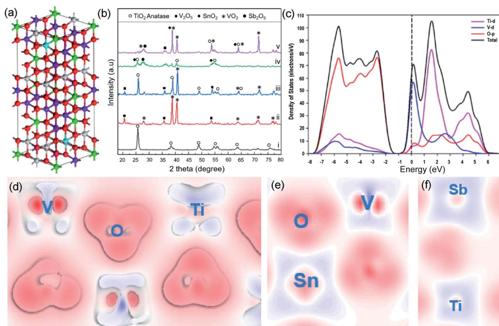
Fig. 12 (a) Schematic of the \text{Ti}_{0.35}\text{V}_{0.35}\text{Sn}_{0.25}\text{Sb}_{0.05} structure. Ti, V, O, Sn and Sb atoms are exhibited in grey, purple, red, green, and cyan balls, respectively. (b) XRD patterns of (i) Ti-oxide; (ii) V-oxide; (iii) \text{Ti}_{0.7}\text{V}_{0.3} -oxides; (iv) \text{Ti}_{0.7}\text{Sn}_{0.25}\text{Sb}_{0.05} -oxides; and (v) \text{Ti}_{0.35}\text{V}_{0.35}\text{Sn}_{0.25}\text{Sb}_{0.05} -oxides after annealing. (c) Projected density of states and band structure \text{Ti}_{0.7}\text{V}_{0.3} . (d) Electron density difference plots of \text{Ti}_{0.7}\text{V}_{0.3} . (e and f) Electron density difference plots of \text{Ti}_{0.35}\text{V}_{0.35}\text{Sn}_{0.25}\text{Sb}_{0.05} structures. The depletion of electrons presented by blue areas, and the electron accumulation by red areas. Reproduced with permission. 77 Copyright 2020, Elsevier.
