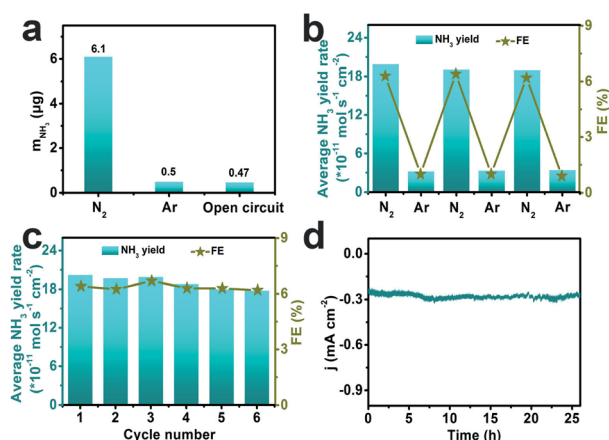
Fig. 3 (a) The amount of \text{NH}_3 produced for \text{Mo}_3\text{Si}/\text{GP} under different electrochemical conditions. (b) \text{NH}_3 yield rate of alternative \text{N}_2 -saturated and Ar-saturated tests at -0.4 V for 2 h. (c) \text{NH}_3 yield rate and FE of cycling tests at -0.4 V. (d) Time-dependent current density curve of \text{Mo}_3\text{Si}/\text{GP} at -0.4 V for 26 h.
