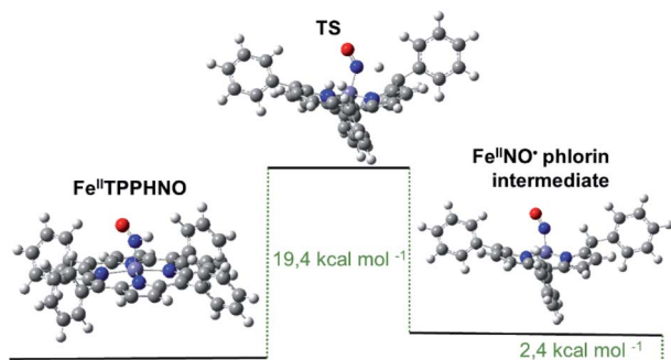
Fig. 2 Optimized structures and calculated energy differences for \text{Fe(II)TPP(HNO)} , the final phlorin intermediate and transition state.
