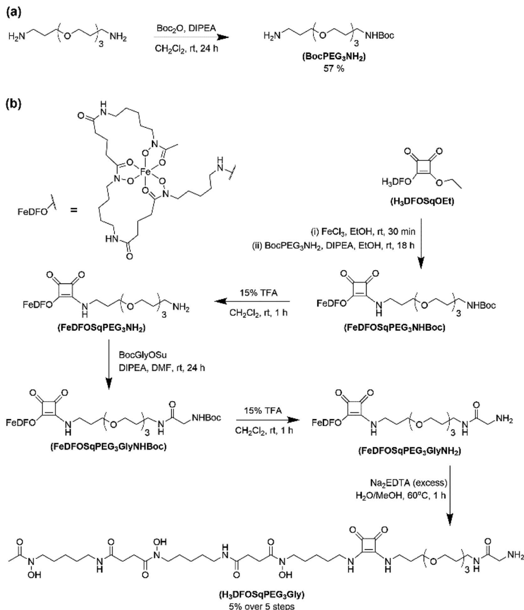
Fig. 3 Reaction scheme for the synthesis of (a) compound 1 and (b) \text{H}_3\text{L}^1 .
