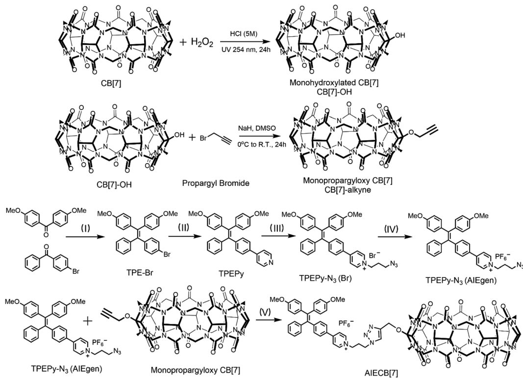
Scheme 2 The Synthetic route for AIECB[7]. Reagents and conditions: (I) \text{TiCl}_4 , Zn dust, anhydrous THF, -78^\circ\text{C} , and 24 h; (II) 4-pyridinylboronic acid, \text{Pd}(\text{PPh}_3)_4 , TBAB, 2M \text{K}_2\text{CO}_3 (aq), THF, 80^\circ\text{C} , and 5 h; (III) 1-azido-3-bromopropane, DMF, 100^\circ\text{C} , and 12 h; (IV) \text{KPF}_6 ; (V) \text{CuSO}_4 , sodium ascorbate, DMSO, 80^\circ\text{C} , and 24 h.
