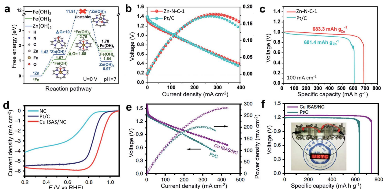
Fig. 11 (a) Free-energy diagrams for Zn(OH) 2 , Fe(OH) 2 , and Fe(OH) 3 during the metal corrosion process, as based on the M-N 4 (M = Zn/Fe) structure. (b) Discharging polarization and the corresponding power density curves of a primary Zn-air battery at a scan rate of 5 mV s -1 . (c) Discharge curves of the Zn-air battery at 100 mA cm -2 discharge rate. Reproduced by permission. 106 Copyright 2019, Wiley-VCH. (d) Linear sweep voltammetry (LSV) curves of NC, Cu ISAS/NC and Pt/C catalysts. (e) Polarization and corresponding power density plots. (f) Specific capacity at 50 mA cm -2 . (Inset: a photograph showing light-emitting diode panel powered by three Cu ISAS/NC-based Zn-air batteries). Reproduced by permission. 112 Copyright 2019, Springer Nature.
