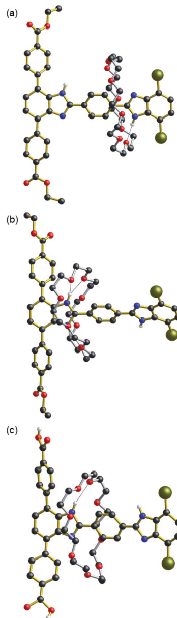
Fig. 2 Ball-and-stick representations of the single-crystal X-ray structures of (a) neutral [\text{2}]\text{rotaxane} diester 2 , (b) protonated [\text{2}]\text{rotaxane} diester [\text{H}2\text{C}24\text{C}8][\text{BF}_4] and (c) neutral [\text{2}]\text{rotaxane} diacid 3 . Colour key: green = bromine, red = oxygen, blue = nitrogen, black = carbon, white = hydrogen. \text{BF}_4 anions, solvent molecules and H-atoms not involved in primary H-bonds are omitted for clarity.
