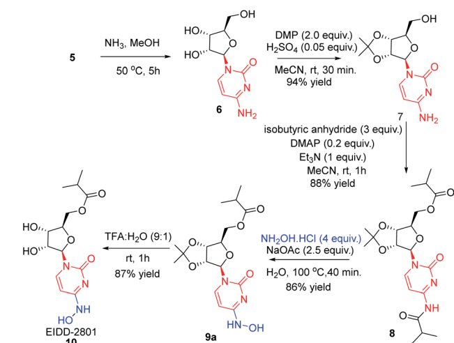
Scheme 4 Diester synthesis and regioselective conversion of N -hydroxylaton.
