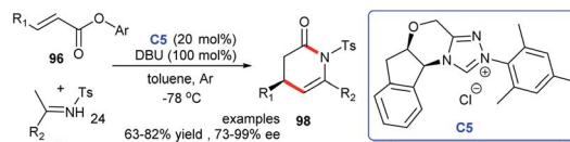
Scheme 30 The synthesis of δ-lactams.
