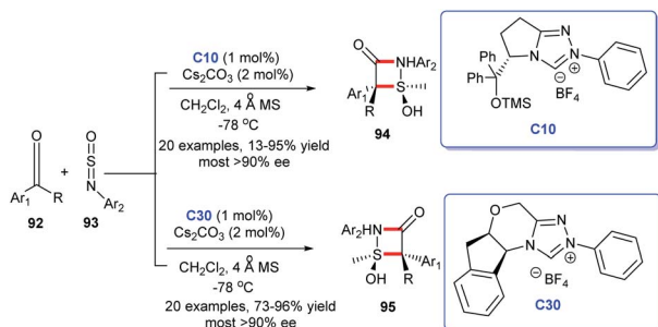
Scheme 29 The synthesis of β-lactams.
