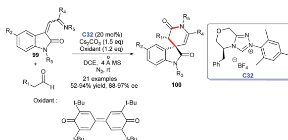
Scheme 31 The synthesis of oxindole δ-lactams.
