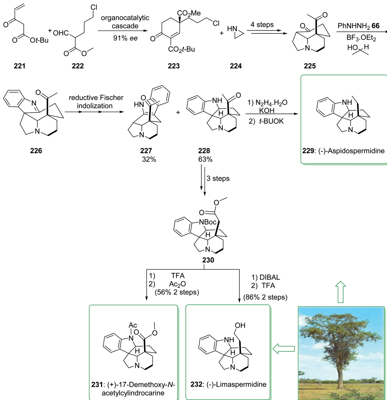
Scheme 29 Total synthesis of (–)-aspidospermidine ( 229 ), (+)-17-demethoxy- N -acetylcylindrocaryne ( 231 ) and (–)-limaspermidine ( 232 ).
