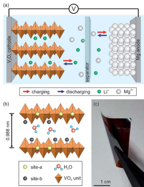
Fig. 1 (a) Schematic depiction of the design and working principle of the hybrid batteries using a dual-salt electrolyte and Mg anode. The working principle includes the de-intercalation of Li + from the cathode and the deposition of Mg 2+ on the Mg anode during charging. For the discharging process the reactions are vice versa . (b) Scheme of the V 2 O 5 bilayer with its intercalation sites, site-a and site-b, the incorporated water molecules assuring that the interlayer distance is large enough to enable ion intercalation. (c) Digital image showing the high flexibility of the self-supporting V 2 O 5 nanofiber-based cathode.
