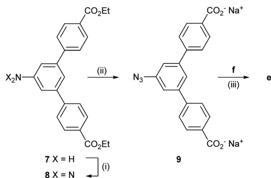
Scheme 4 Synthesis of the stopper 9 in 2 steps and CuAAC "click" reaction providing e . Reagents and conditions: (i) TMSN 3 , tBuONO, DMF, 0 °C to rt, 6 h, 98%; (ii) NaOH, THF-MeOH-H 2 O (4:4:1), 50 °C, 1 h, 86%; (iii) CuSO 4 ·5H 2 O, sodium ascorbate, H 2 O-MeOH (2:1), rt, 1 h, 65%.
