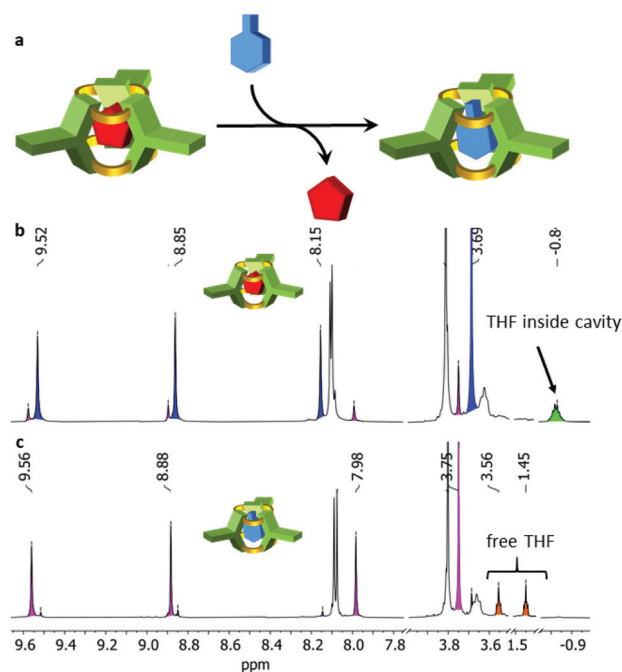
Fig. 6 (a) Exchange of host molecules from THF@( R,R )- 9 to toluene- d 8 @( R,R )- 9 . (b) 1 H NMR spectrum (700 MHz) of freshly prepared THF@( R,R )- 9 in toluene- d 8 . (c) same sample after exchange of THF guest by toluene- d 8 . Note, that in the upper spectrum some toluene- d 8 @( R,R )- 9 has formed.
