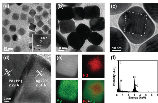
Fig. 1 Structural characterization of Pd Octs and Pd@Ag cubes. (a) TEM image of Pd Octs. (b and c) TEM and (d) HR-TEM images, (e) elemental mapping (raw data are displayed as Fig. S1, ESI † ) and (f) the corresponding EDS profile of a Pd@Ag cube.
