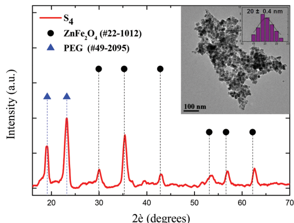
Fig. 1 All the peaks of the XRD pattern are well-matched with the standard JCPDS data of \text{ZnFe}_2\text{O}_4 , while the two distinct peaks at 19^\circ and 23^\circ confirm the presence and crystallization of PEG on the surface. The bright-field TEM image of the sample ( S_4 ) clearly shows nearly spherical nanoparticles covered by PEG.
