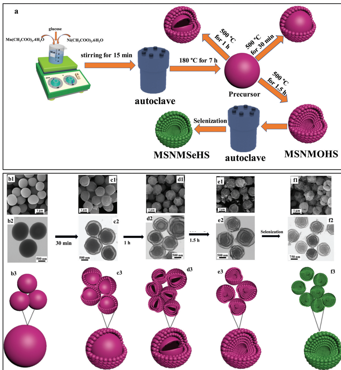
Fig. 1 (a) The schematic fabrication process of the MSNMs. (b1–b3) FE-SEM image, TEM image and the corresponding schematic illustration of the MAPs before thermal treatment. (c1–c3) FE-SEM image, TEM image and the corresponding schematic illustration of the MAPs after thermal treatment at 500^\circ\text{C} for 30 min. (d1–d3) FE-SEM image, TEM image and the corresponding schematic illustration of the MAPs after thermal treatment at 500^\circ\text{C} for 1 h. (e1–e3) FE-SEM image, TEM image and the corresponding schematic illustration of the MAPs after thermal treatment at 500^\circ\text{C} for 1.5 h. (f1–f3) FE-SEM image, TEM image and the corresponding schematic illustration of the MSNMs.
