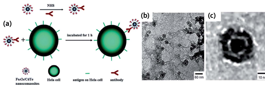
Fig. 6 (a) Schematic design of immuno-labeling by Fe 3 O 4 /CdTe nanocomposites. (b and c) TEM image of Fe 3 O 4 /CdTe MNFPs. Reproduced from ref. 2 with permission from American Chemical Society, copyright 2010.
