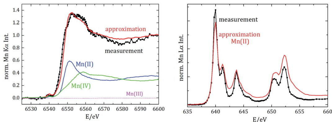
Fig. 5 Results of the linear combination of reference spectra to approximate the spectrum of the aged anode (left: for the K-edge NEXAFS analysis; right: for the L_2 , L_3 edge NEXAFS). The measurement of the aged anode is shown in black, and the best approximation in red. While the spectrum of L-edge NEXAFS is best approximated by divalent manganese solely, the K-edge approximation is composed of di- and tetra-valent components (blue and green graphs).
