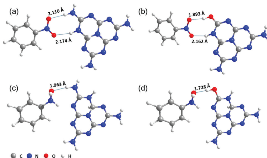
Fig. 4 Analysis of the reaction mechanism. The optimized adsorption status of NB and PHA over PCN (a and c) and –OH-modified PCN (b and d). The numbers in the figure represent the lengths of the hydrogen bonds.
