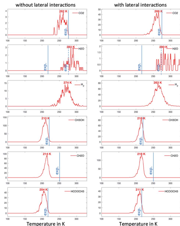
Fig. 5 TPO spectra of methanol on Au(111) for scenario #2. Temperature ramp is 10 \text{ K s}^{-1} . The initial coverages are: 0.1 ML of \text{CH}_3\text{O} and 0.02 ML in O.
