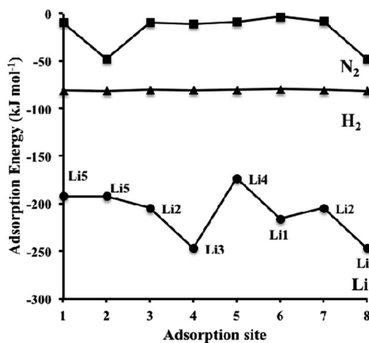
Fig. 8 Dispersion-corrected (revPBE-D3) adsorption energies of Li (circles), H 2 (triangles) and N 2 (squares) over the symmetry unique adsorption sites on \eta -Mn 3 N 2 depicted in Scheme 1 (for H 2 and N 2 ). The data for Li corresponds to the adsorption site configuration depicted in Scheme 2. Lines connecting the data points have been drawn to guide the eye.
