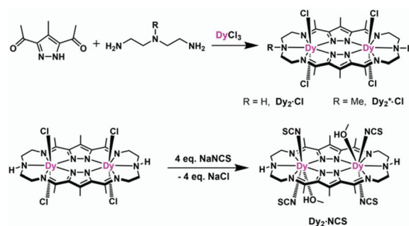
Scheme 2 Schematic drawing of the assemblies of \text{Dy}_2^*\text{Cl} , \text{Dy}_2^*\text{Cl} , and \text{Dy}_2^*\text{SCN} .
