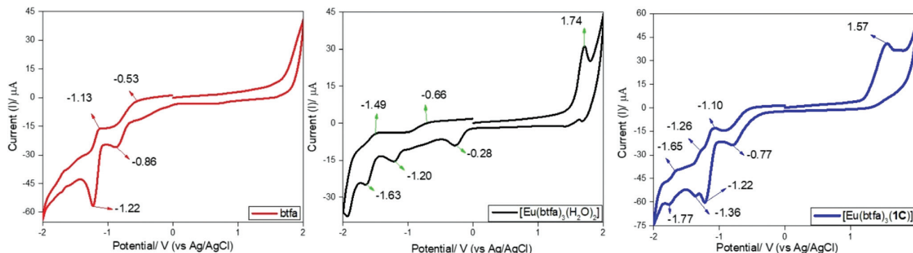
Fig. 7 Cyclic voltammograms of btfa (red), [Eu(btfa) 3 (H 2 O) 2 ] (black) and [Eu(btfa) 3 1c] (blue) in the region between -2.0 to 2.0 V on glassy carbon electrode in 0.1 M Bu 4 NPF 6 solution in DCM at a scan rate of 100 mV s -1 .
