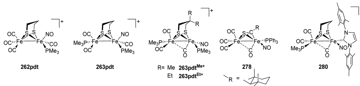
Fig. 85 Exemplary nitrosyl substituted complexes. Note: in the crystalline state 263\text{pdt} shows different degrees of rotation.
